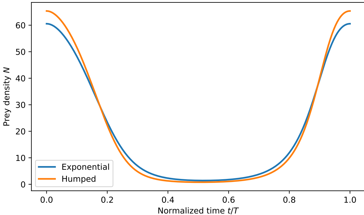
Prey density N over one periodic cycle
