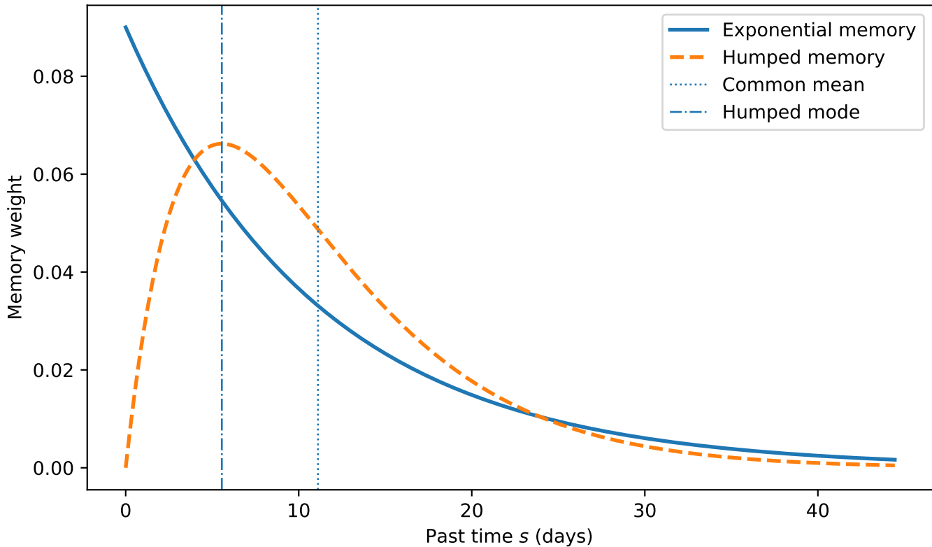
Memory kernels with the same mean response time
