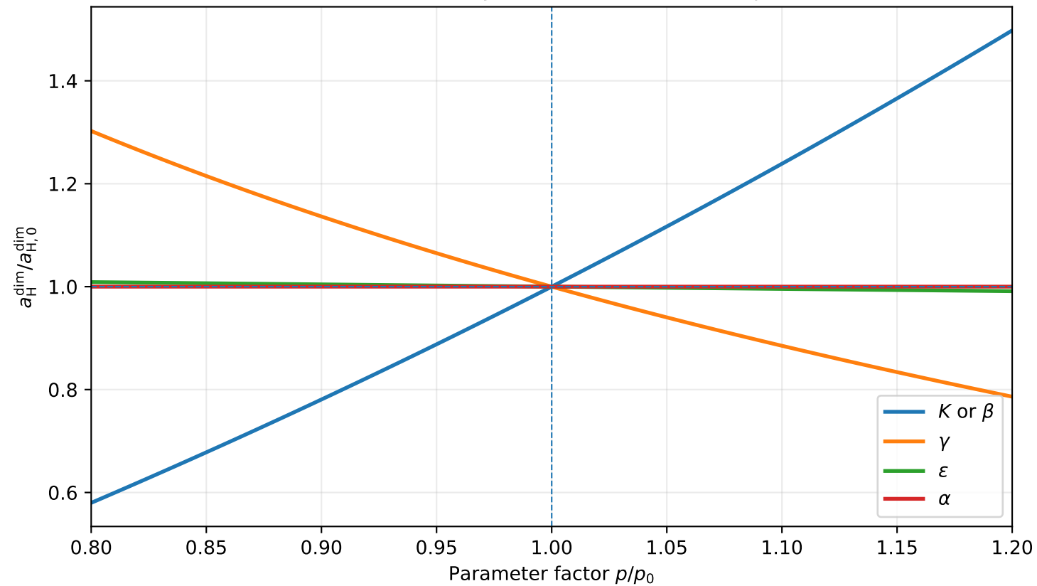
One-at-a-time sensitivity of the dimensional Hopf threshold
