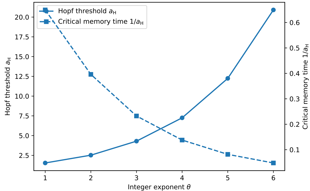
Threshold variation in f_\theta(n) = 1 - n^\theta
