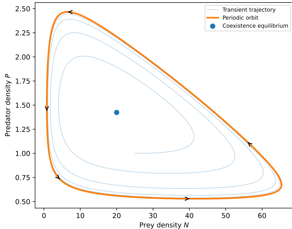
Projected orbit, a = 0.18 < a_H
