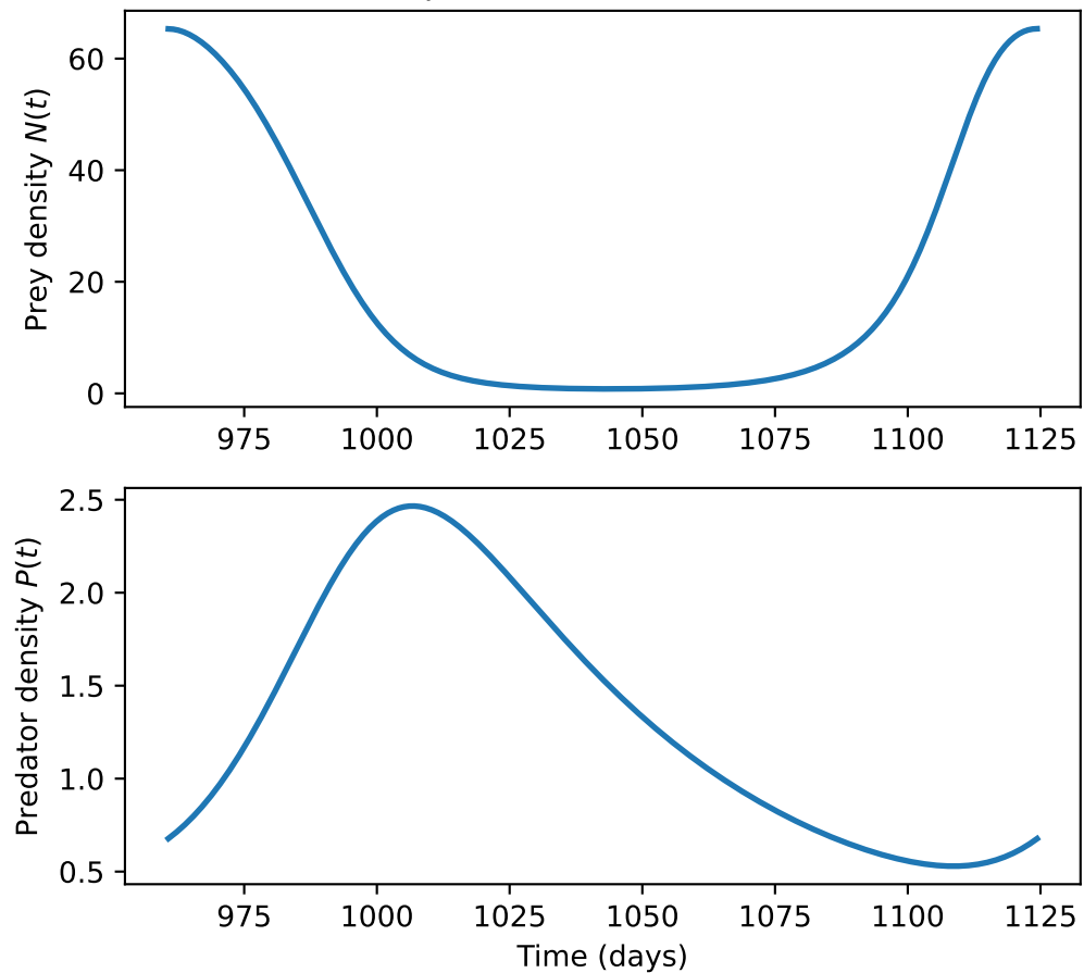
One period after the transient
