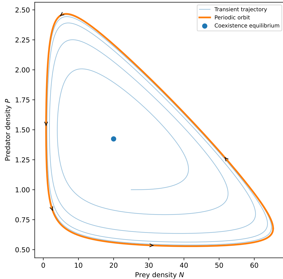
Projected orbit, a = 0.18 < a_H
