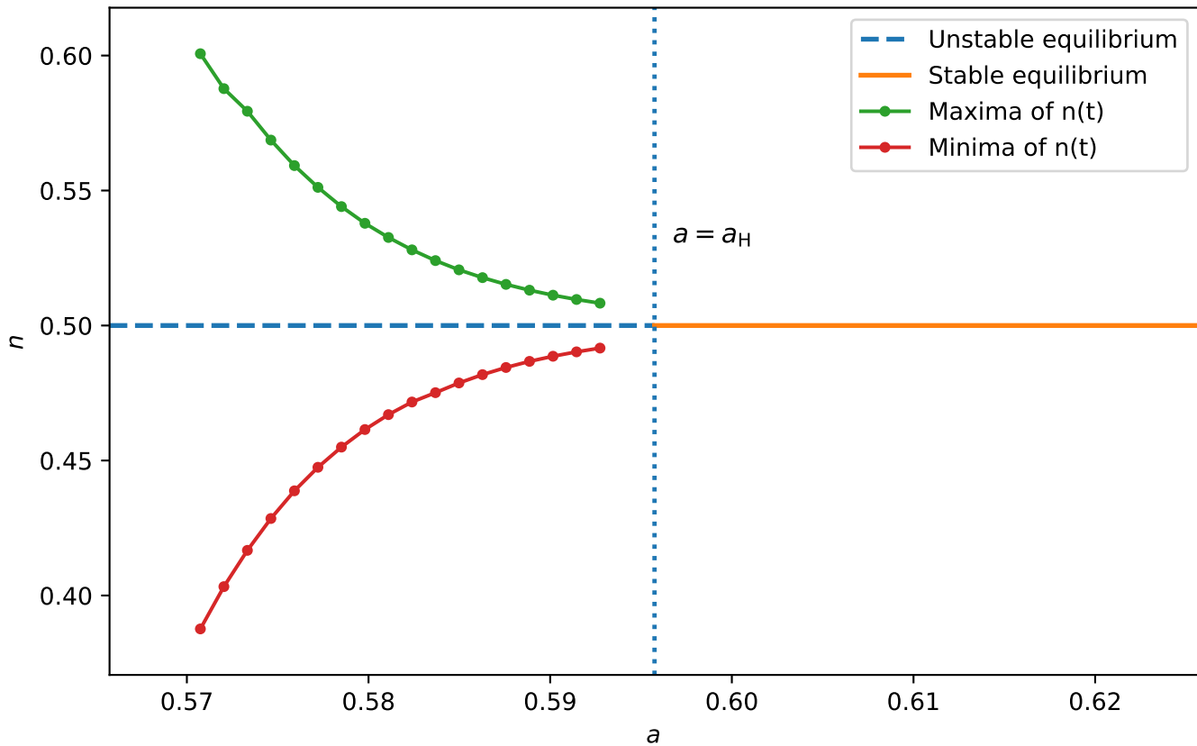
Local bifurcation diagram: hyperlogistic case
