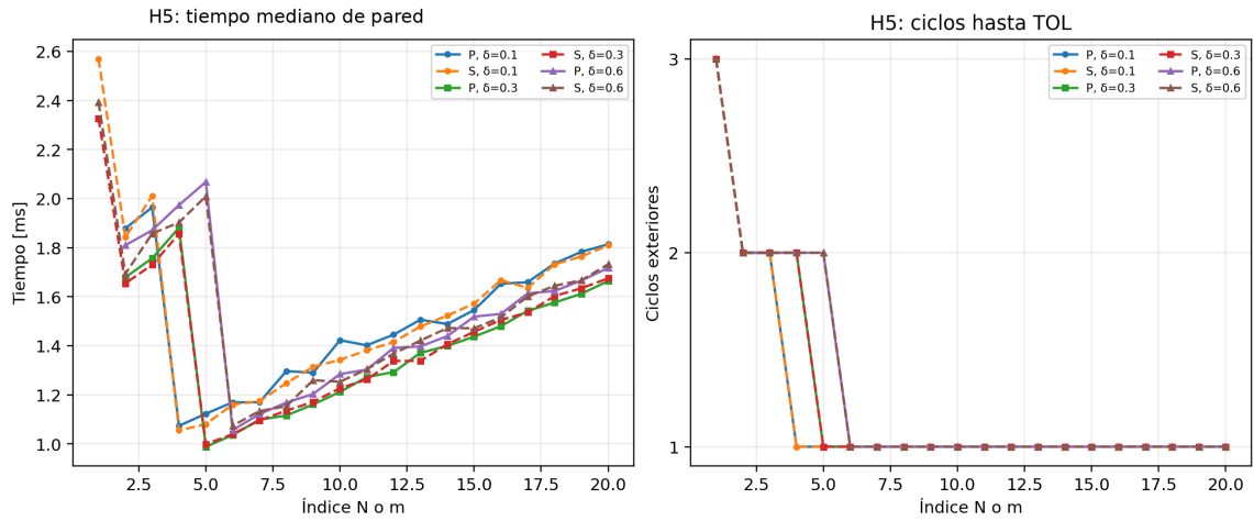
Figure S4: Complete sweep in H_5 for three initial distances. Left: median elapsed wall time. Right: number of outer cycles required to reach TOL = 10^{-12} . The first cycle of P_N and S_N has the same resources. With more than one cycle, memory is active, but that activation does not imply a resolved timing separation; the curves are interpreted together with the IQRs in this supplement.
