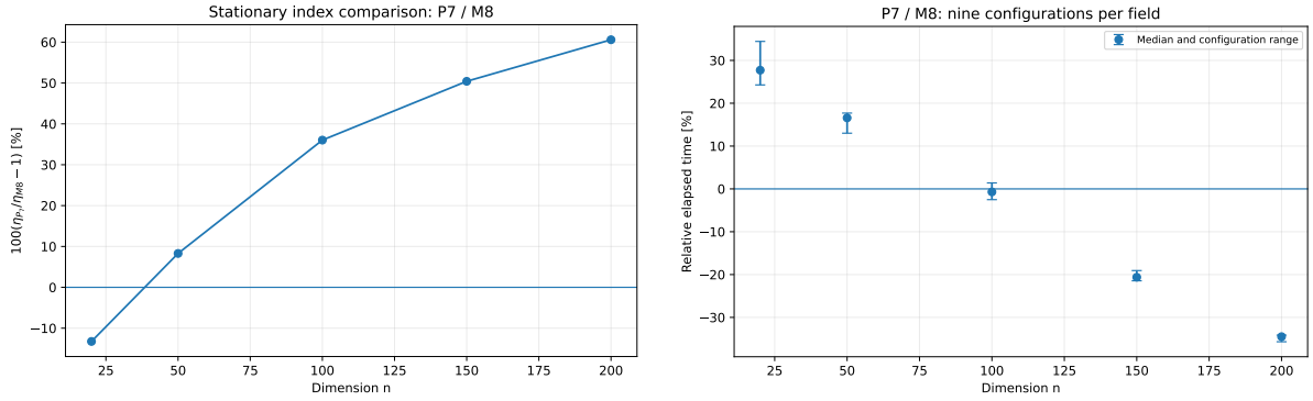
Figure S1: P_7/M_8 : stationary index advantage (left) and median with configuration range of relative elapsed time (right). Positive index differences and negative time differences favor P_7 . The displayed range is not an IQR or confidence interval.
