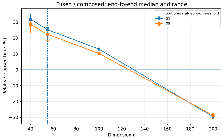
Figure S2: End-to-end \hat{P}_2/(P_2 \circ P_2) : median and range of relative elapsed time. The line n = 55 marks the stationary algebraic threshold, not an estimated temporal crossover. No interpolation establishes universal monotonicity.
