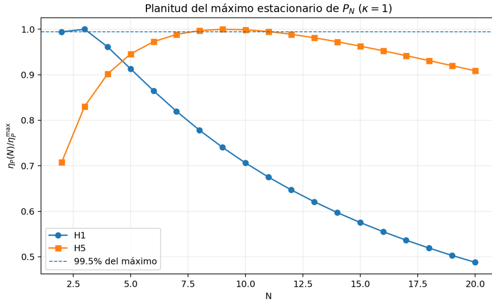
Figure S3: Normalized stationary index of P_N for \kappa = 1 . The dashed line represents 99.5% of the maximum. In H_1 , only P_3 belongs to that band; in H_5 , the band contains P_8, P_9, P_{10}, P_{11} .
