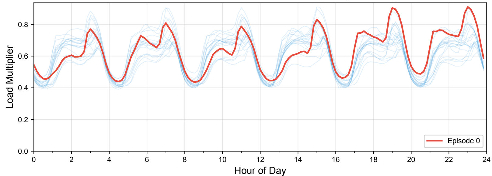
Load "671" Across 20 Episodes (showing daily diversity)
