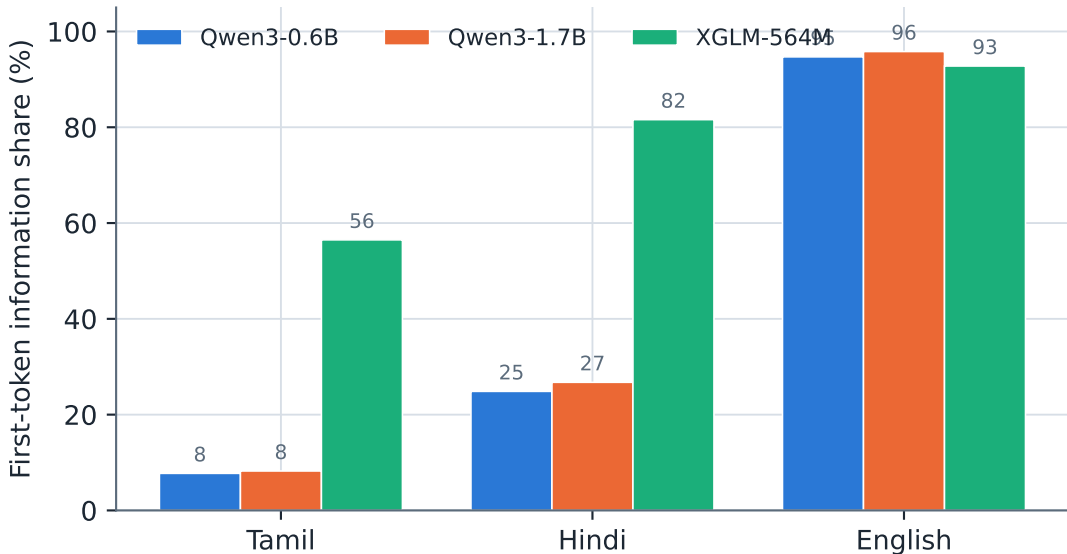
Where a word's information lives: share carried by its first token
