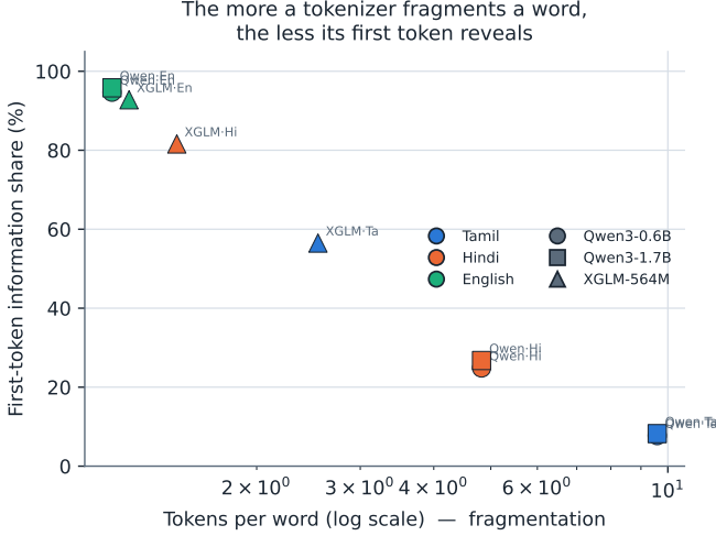
Fig. 5. Across all nine model×language points, the first-token share falls monotonically as the tokenizer fragments the word more. The phenomenon tracks fragmentation, not script: XGLM’s Indic-aware tokenizer (few tokens per word) keeps the information in the first token, like English.
