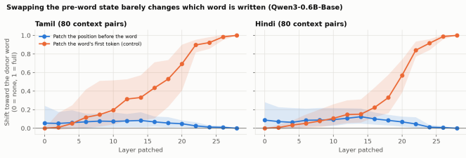
Fig. 8. Activation patching, Qwen3-0.6B. Swapping the pre-word state (blue) barely changes which word is written; swapping the first in-word position (orange control) takes over the decision by the last layer. The word is not localized before it is written.
