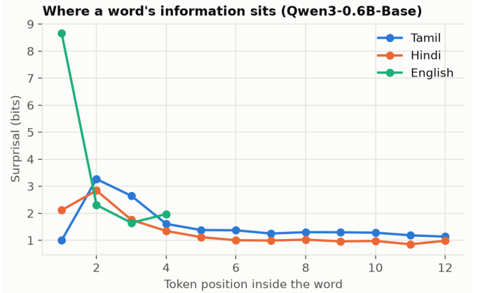
Fig. 4. Mean surprisal (bits) by token position within a word, Qwen3-0.6B. The information of a Tamil/Hindi word is concentrated in its first few interior tokens and then plateaus above zero; an English word is decided at token one.
