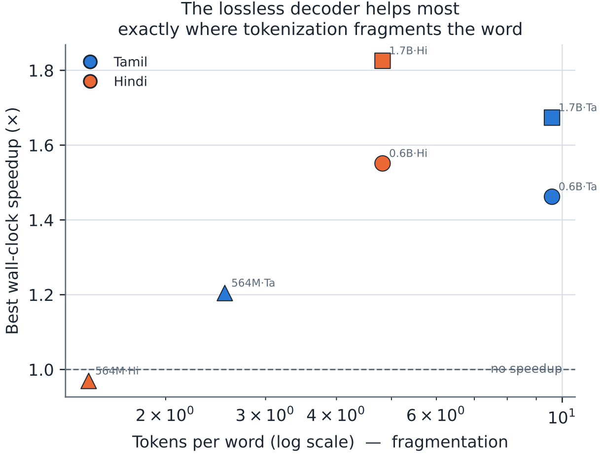
Fig. 15. Best wall-clock speedup against fragmentation, across models and languages. The lossless decoder helps most exactly where the tokenizer fragments the word; where tokenization is already efficient (XGLM) it is roughly neutral.
