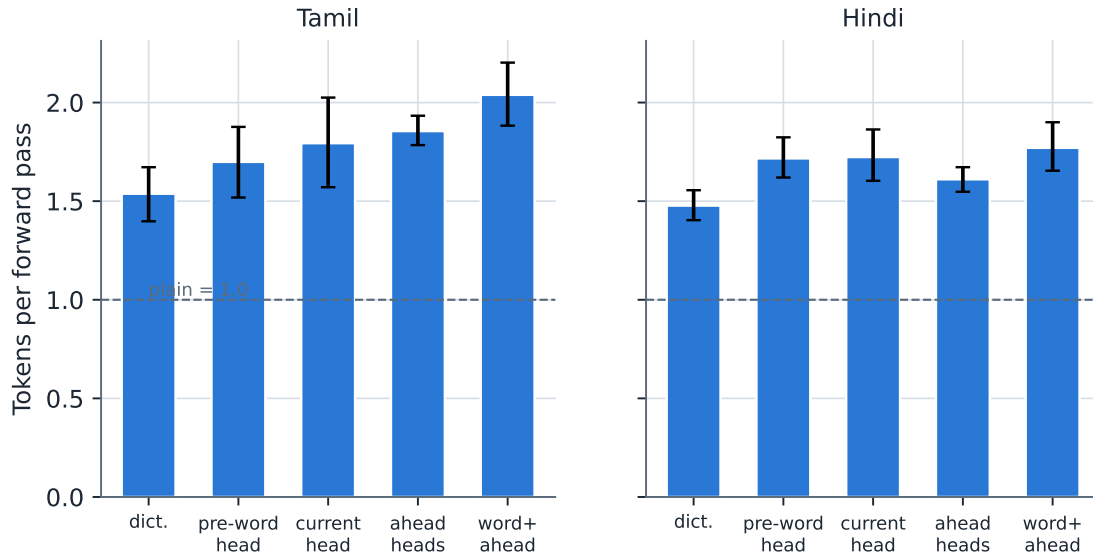
Lossless tokens-per-forward on Qwen3-1.7B (95% bootstrap CI over prompts)
