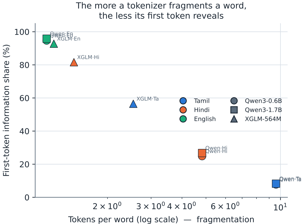
Fig. 5. Across all nine model \times language points, the first-token share falls monotonically as the tokenizer fragments the word more. The phenomenon tracks fragmentation, not script: XGLM’s Indic-aware tokenizer (few tokens per word) keeps the information in the first token, like English.
