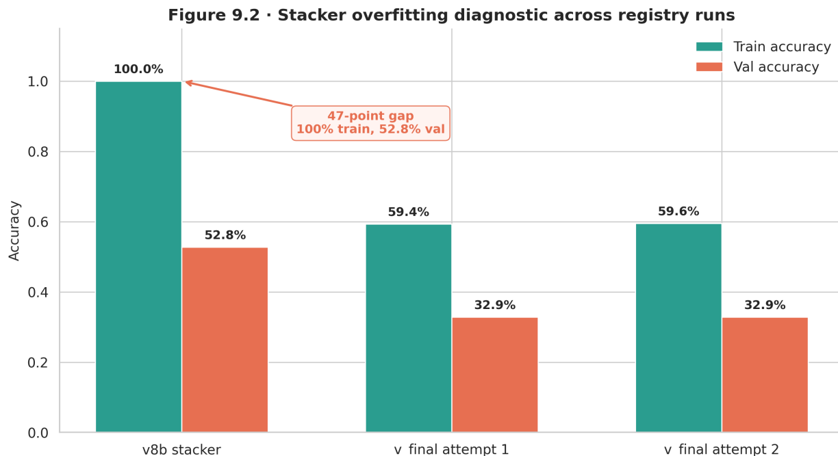
Figure 13: Figure 9.2: LightGBM staker overfitting in v8b. Training accuracy reaches 1.0; validation accuracy plateaus at 0.528 and declines. The 47-point gap indicates memorization.
