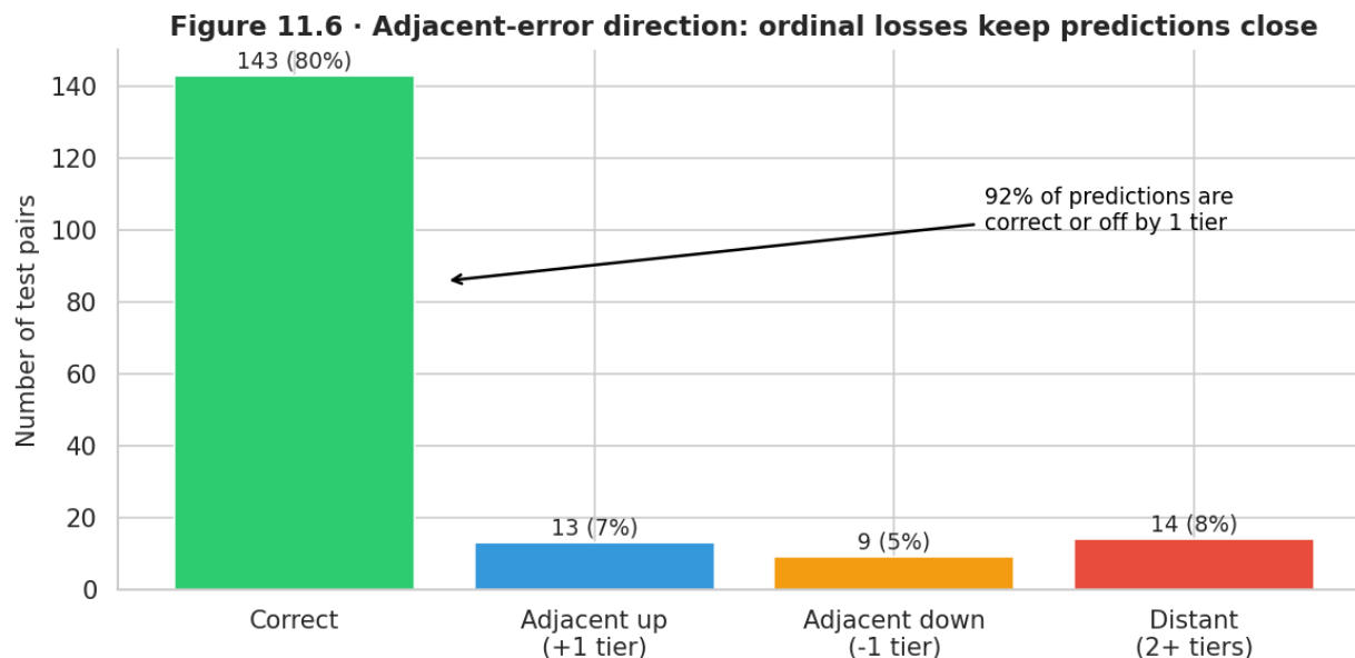
Figure 22: Figure 11.6: Adjacent vs. non-adjacent error breakdown for v_final . The majority of misclassifications are off by one ordinal tier; large errors (two or more tiers) are uncommon.
