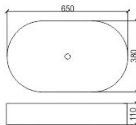
KARAT WASH BASIN Size: 650 x 380 x 110 mm
