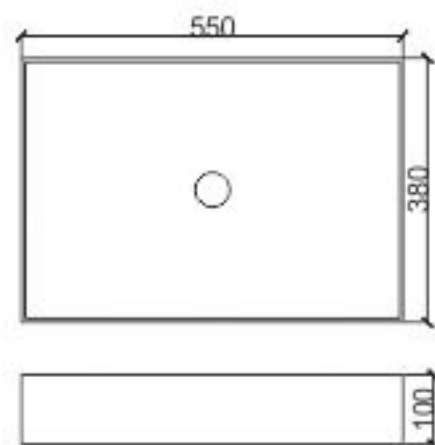
LINE WASH BASIN Size: 550 x 380 x 100 mm
