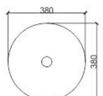
OPTUS WASH BASIN Size: 380 x 380 x 430 mm
