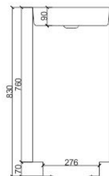
CANBERA WASH BASIN Size: 378 x 378 x 830 mm
