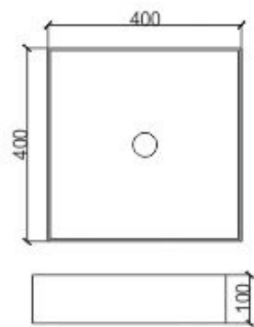
BRAVO WASH BASIN Size: 400 x 400 x 100 mm
