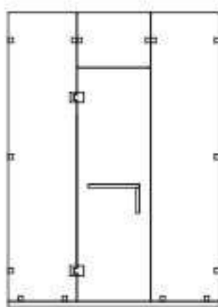
STRAIGHT (3 FIX + 1 DOOR)
