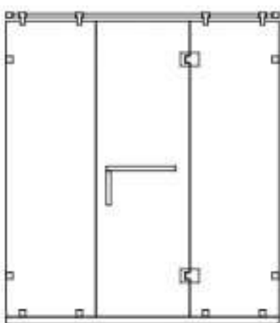
STRAIGHT (2 FIX + 1 DOOR)
