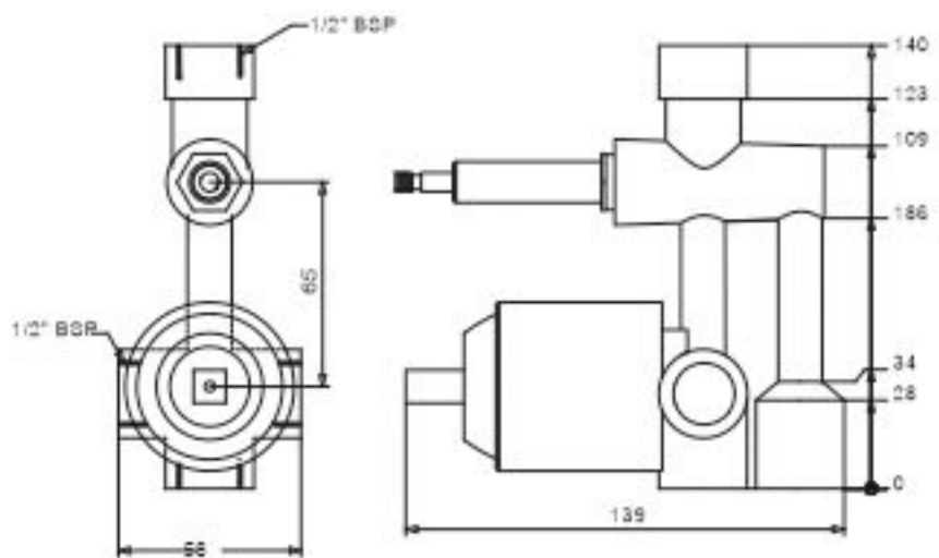
Cat No. : COL-2024 Single Lever Concealed Diverter 3-Inlet Forged Body 46 mm High Flow
