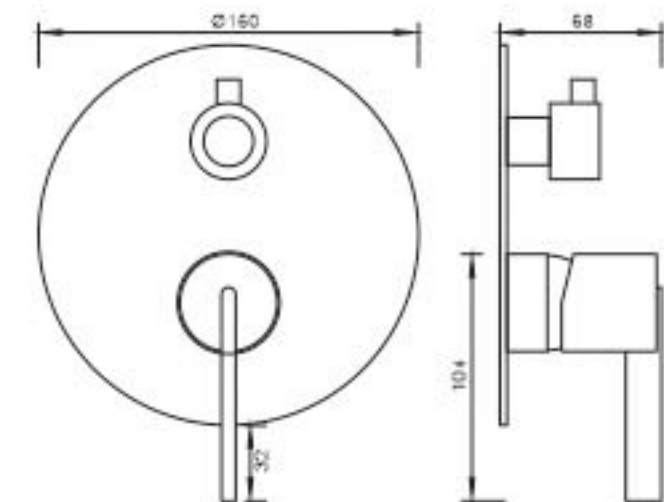
HUBB NICKLE POLISH (2908) Single Lever Concealed Diverter (3 Outlets) with Trim, Handle & Installation Box
