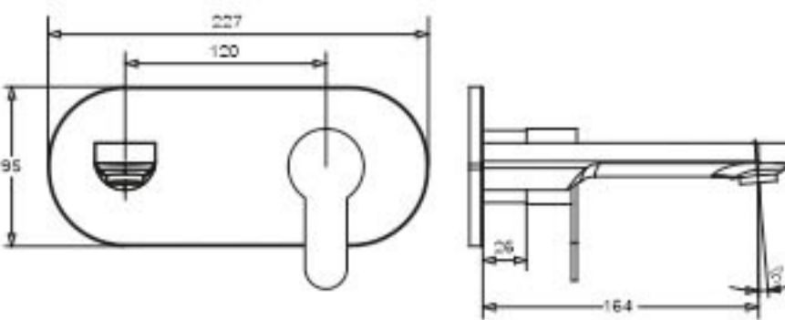
Cat No. : COL-3028 Exposed Part of Single Lever Concealed Basin Mixer Wall Mounted Consisting of Operating Lever, Wall Flange & Spout
