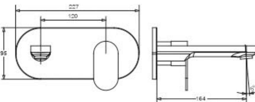
Cat No. : COL-2028 Exposed Part of Single Lever Concealed Basin Mixer Wall Mounted Consisting of Operating Lever, Wall Flange & Spout
