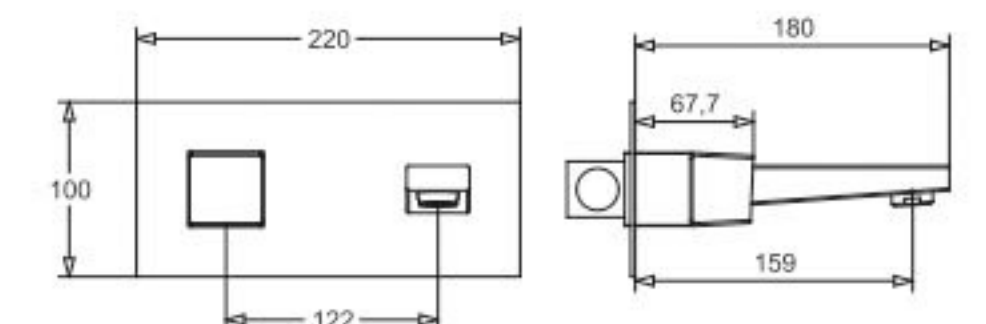
MD-DL8904 (866) Wall Mounted Concealed Basin Mixer with Spout
