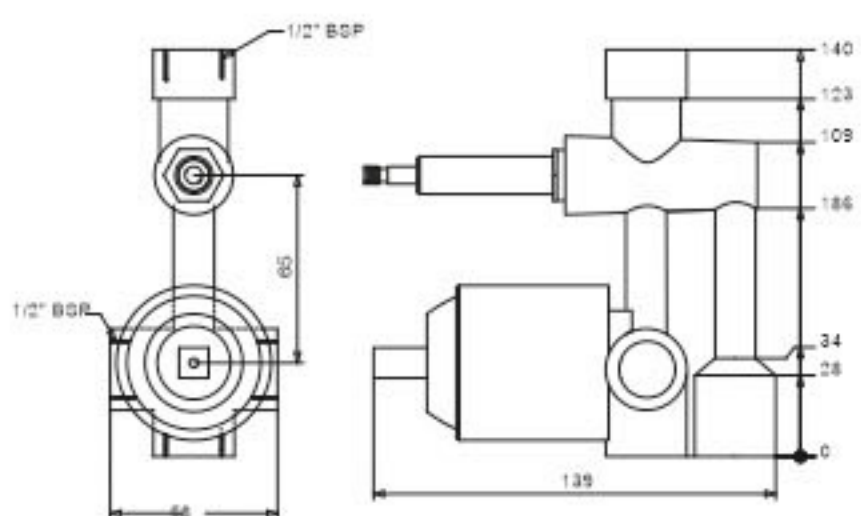
Cat No. : COL-3024 Single Lever Concealed Diverter 3-Inlet Forged Body 46 mm High Flow
