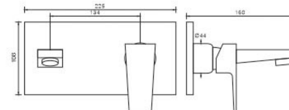
PM-003 (902) Wall Mounted Concealed Basin Mixer
