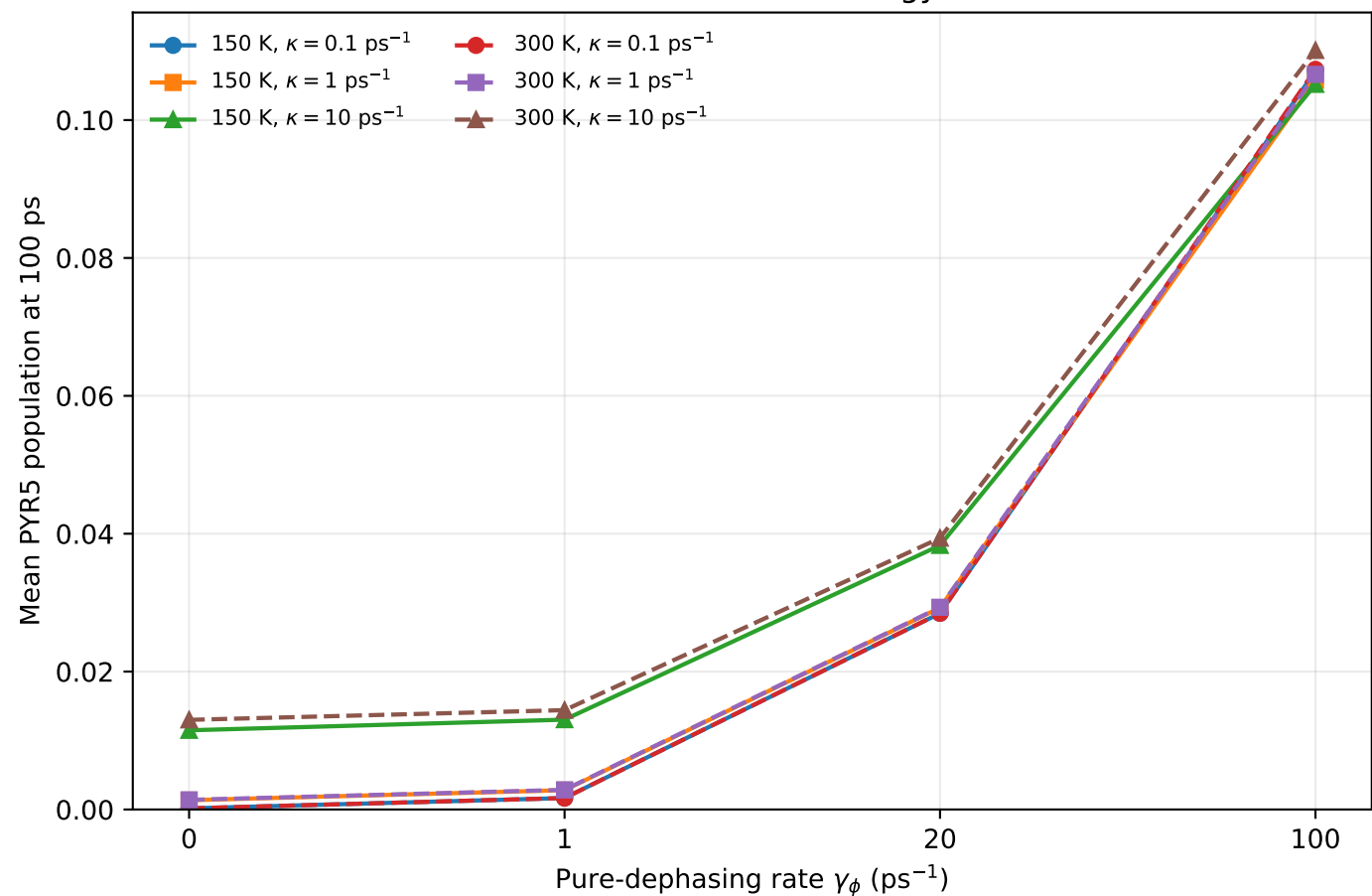
Transient access to the low-energy PYR5 state
