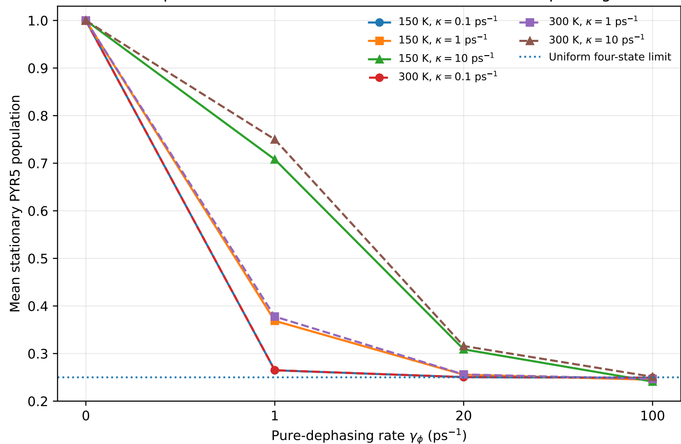
Competition between thermal relaxation and local dephasing
