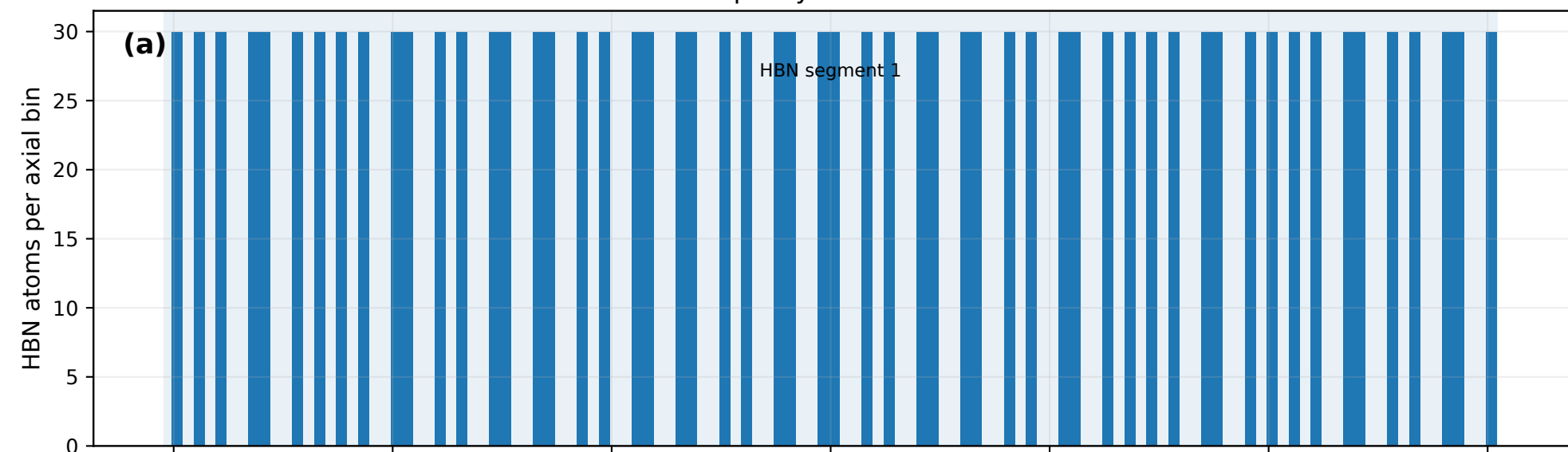
HBN and pyrene geometry in axial-radial space
