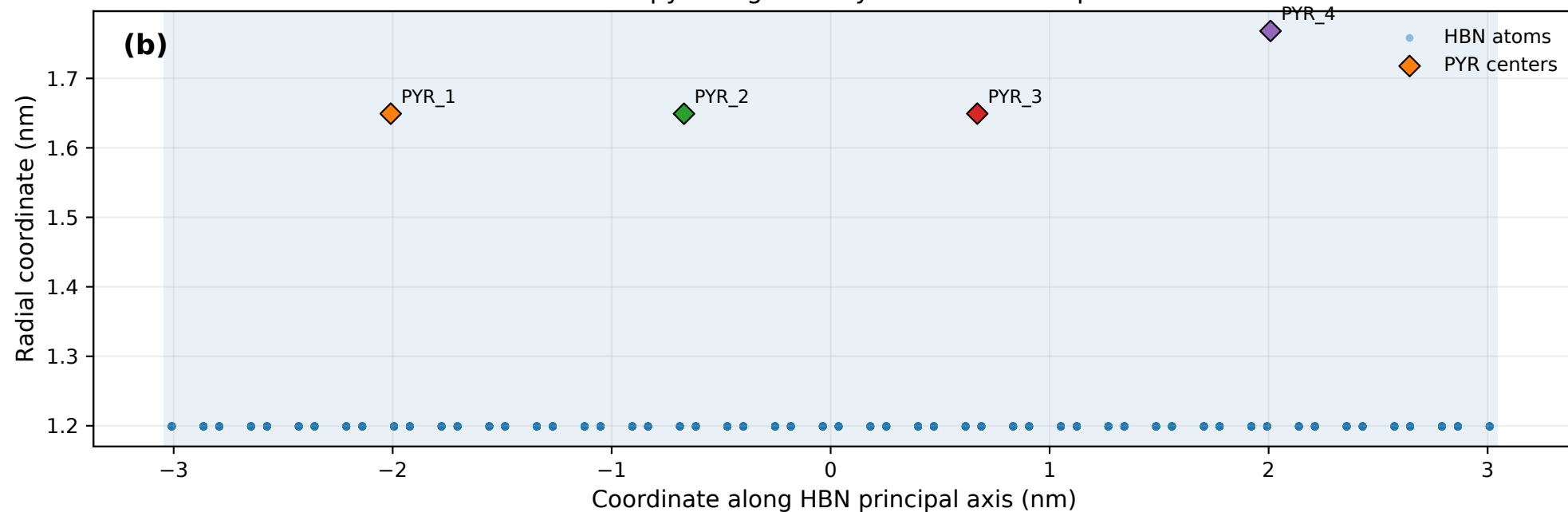
HBN and pyrene geometry in axial-radial space
