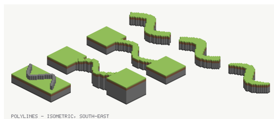
(b) Polyines. The rasterizer splines the points before it offsets the band, so four clicked points draw as a curve.
