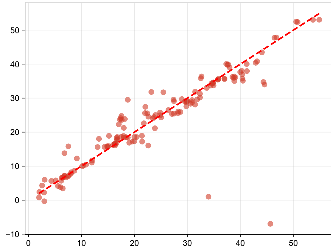
Adam ( R^2 = 0.7866 )
