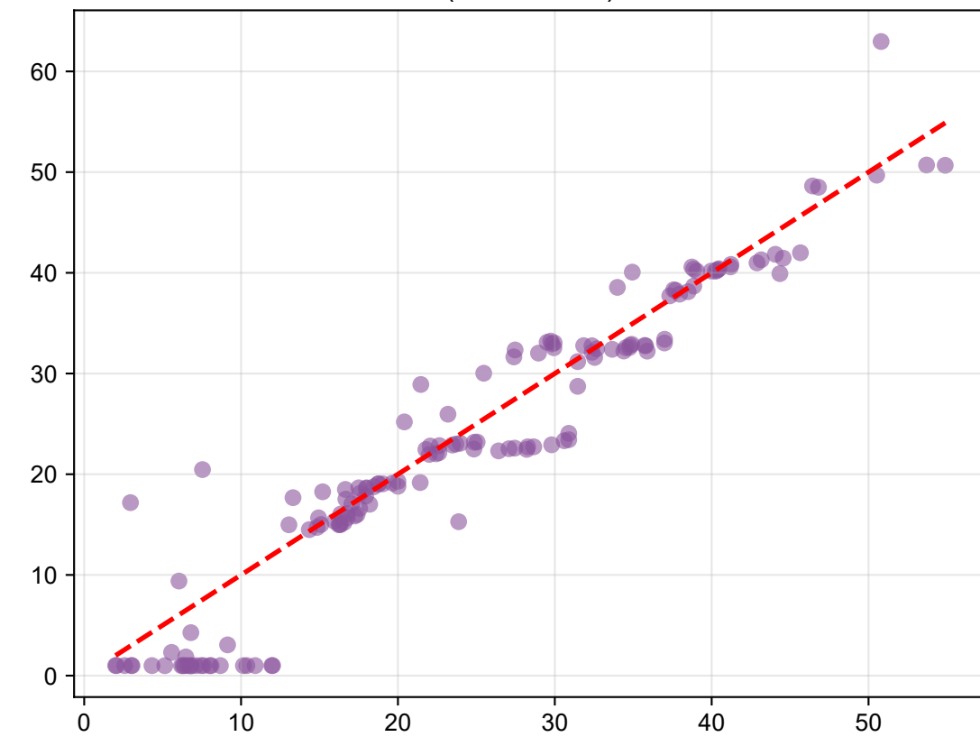
AdaBelief ( R^2 = 0.8941 )
