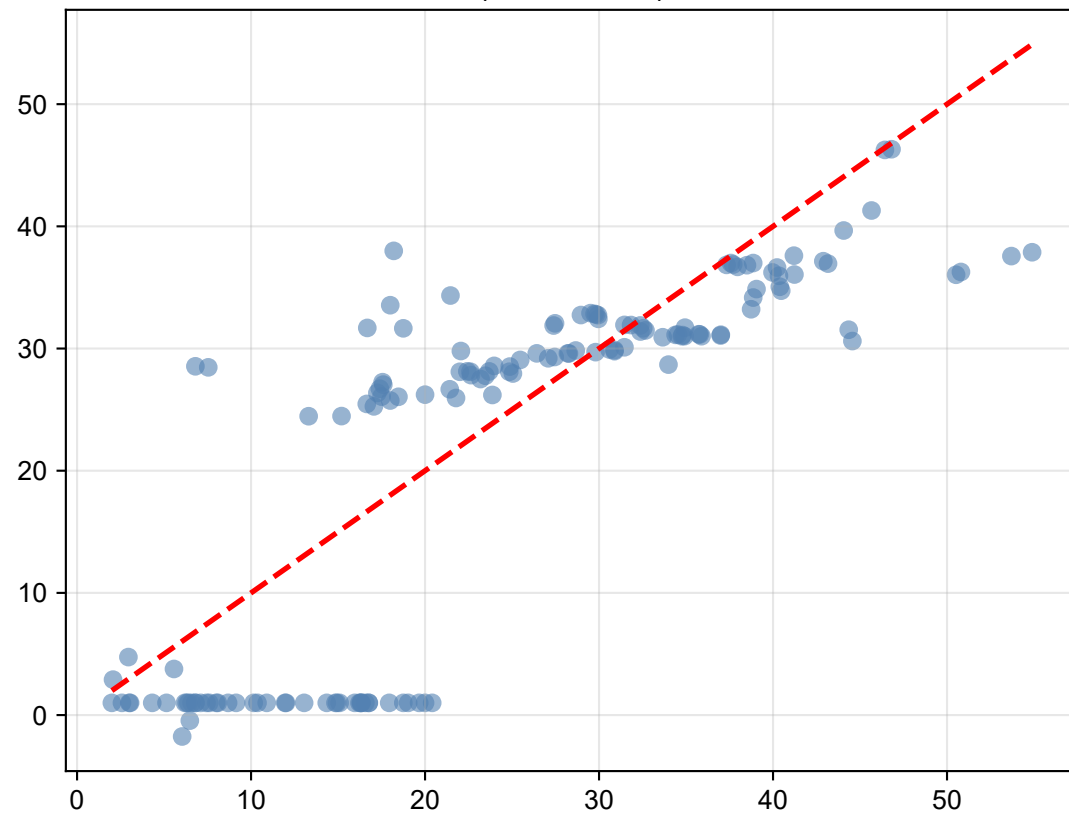
SGD ( R^2 = 0.5297 )
