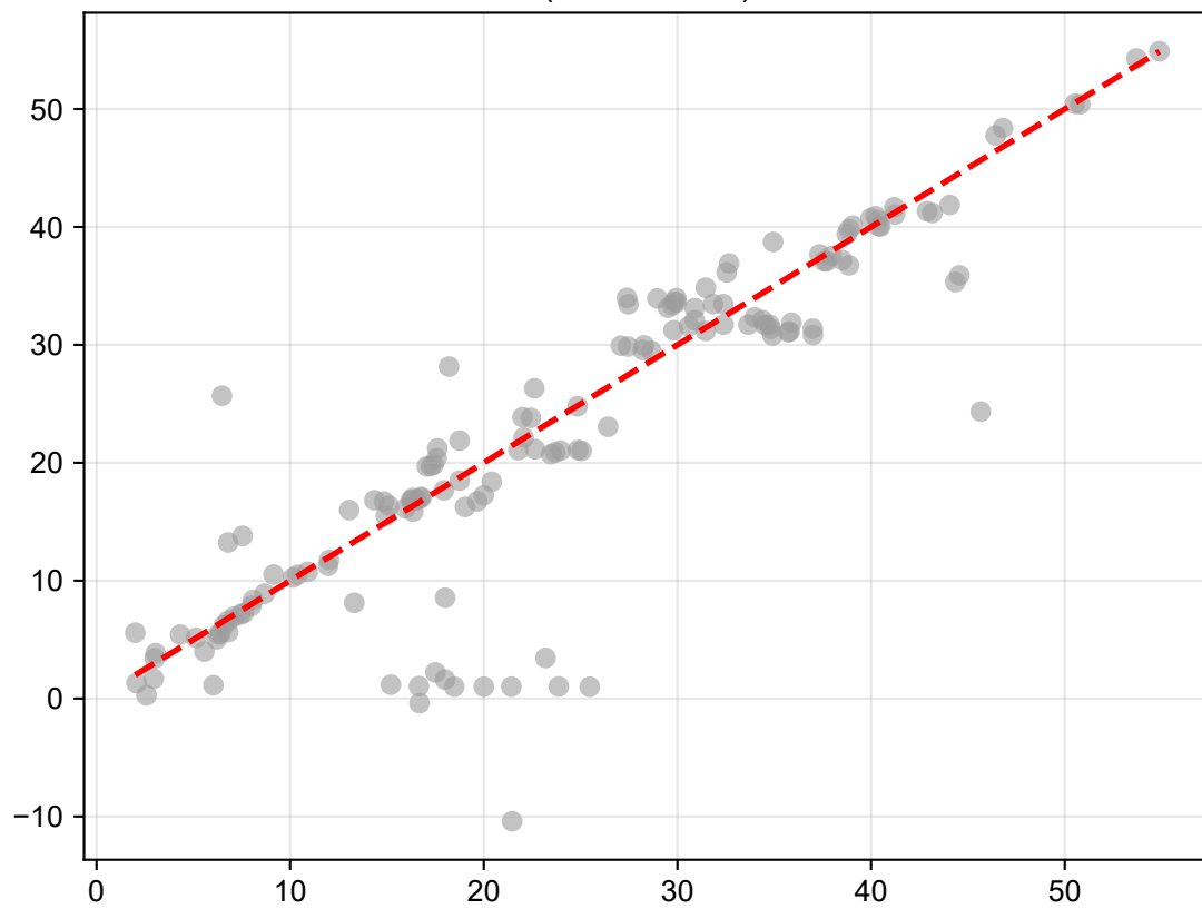
RAdam ( R^2 = 0.7193 )
