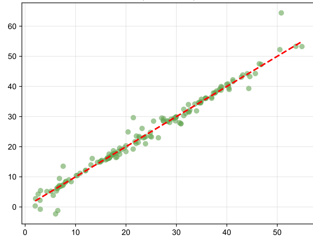
RMSprop ( R^2 = 0.9732 )
