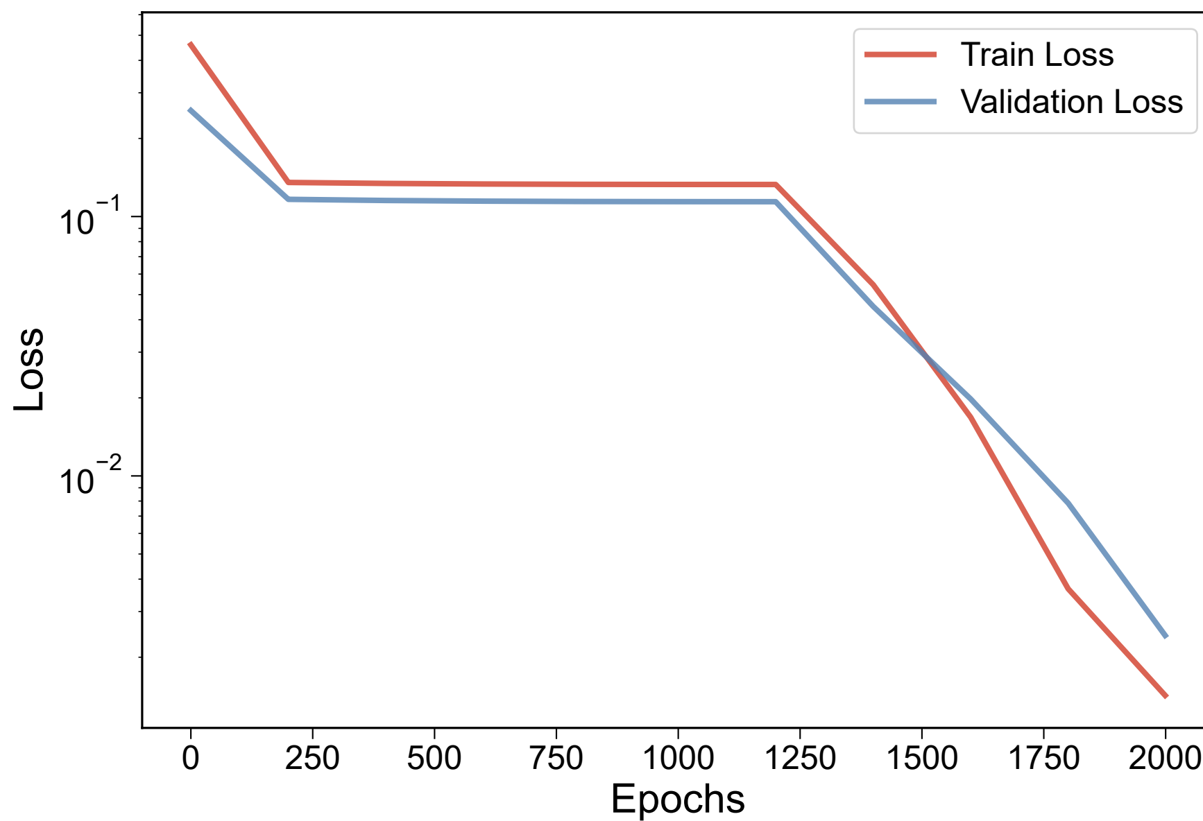
RMSprop Loss Curve
