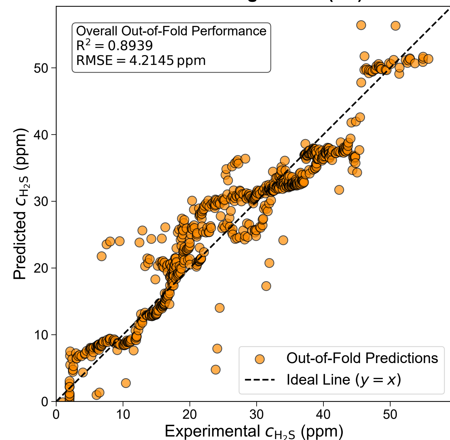
c. Standard ANFIS
