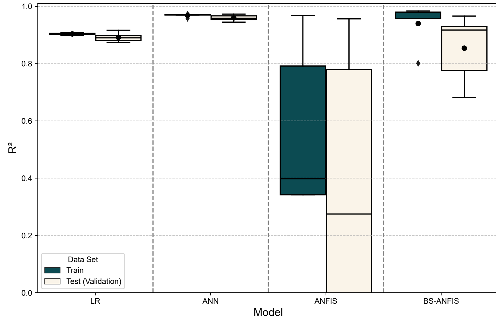
(a) R^2 Score
