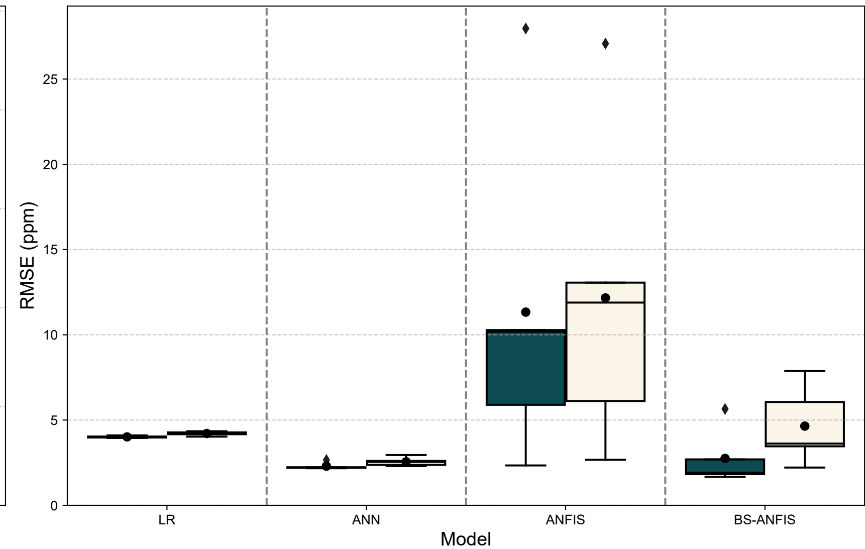
(b) Root Mean Squared Error (RMSE)
