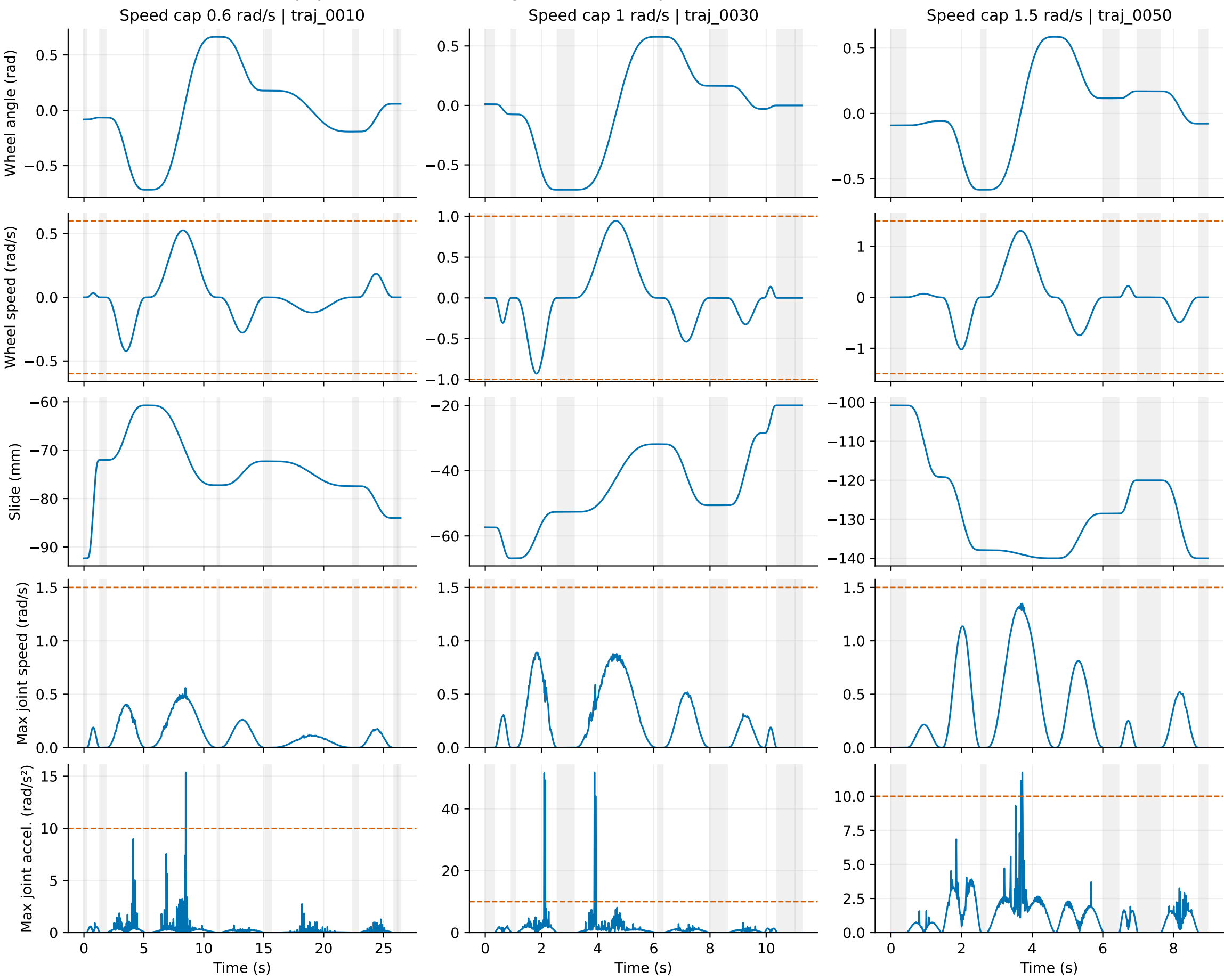
Synthetic random steering— frozen 2-D joint table Gray: pauses; dashed orange: limits; examples selected before audit results
