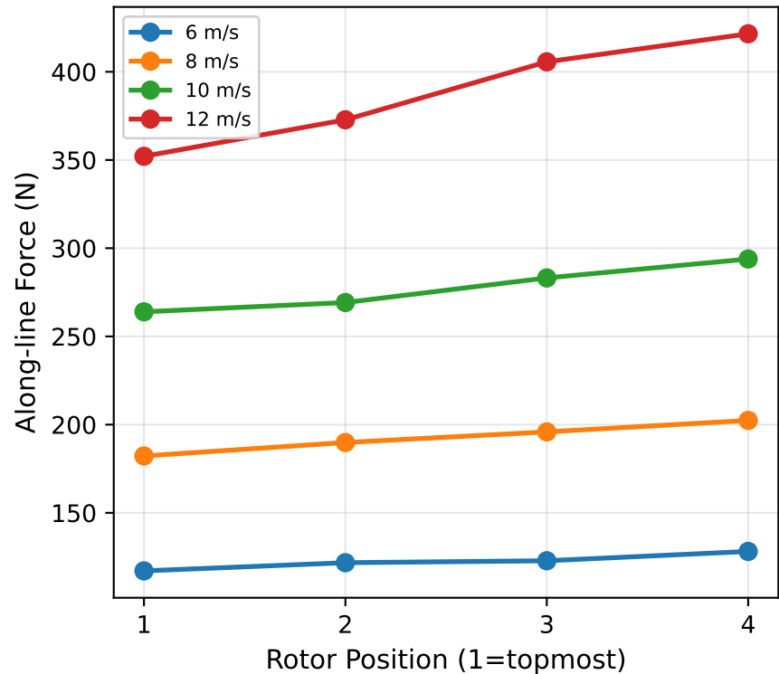
Along-line Force vs Position R=3.0m, N=4, Graded Tilt, 45°
