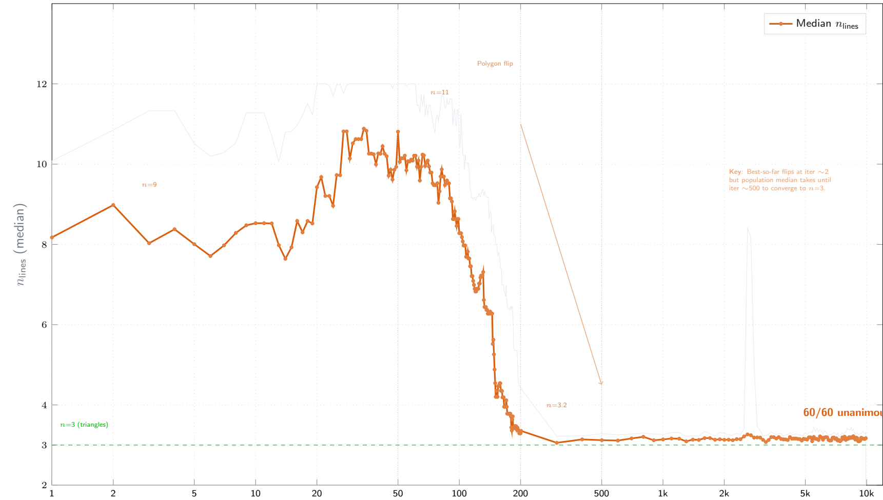
n_{\text{lines}} — Polygon Evolution
