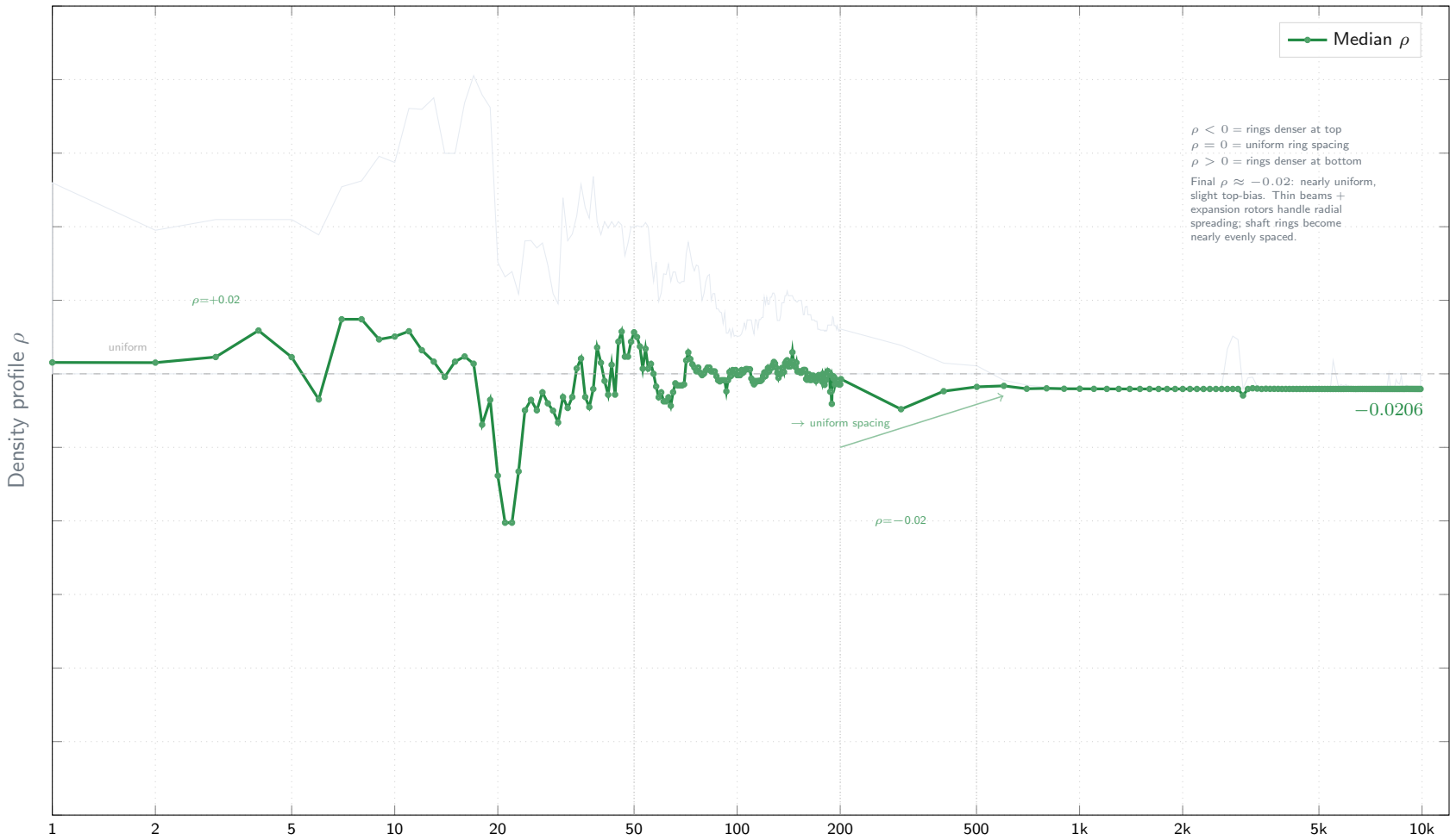
Ring Spacing — Density Profile \rho
