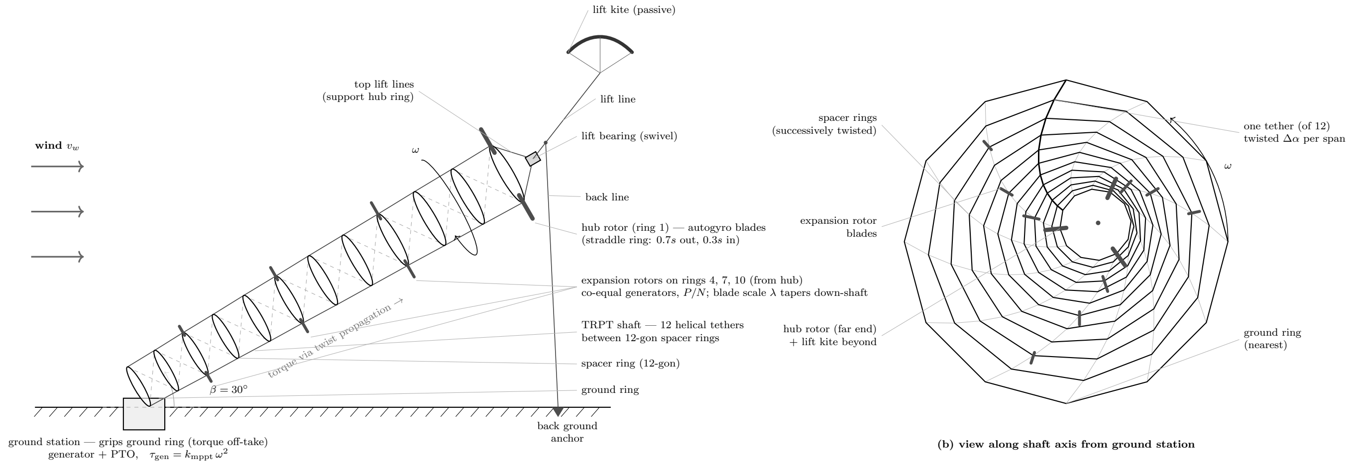
(a) side elevation — wind left \rightarrow right, shaft at \beta = 30^\circ
