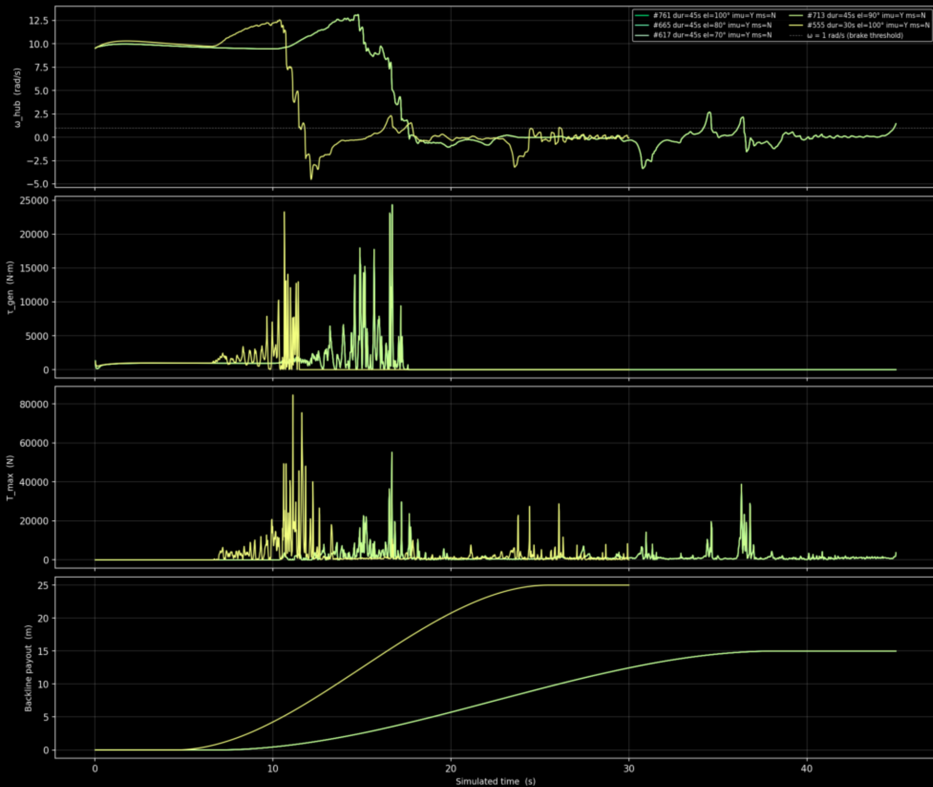
Best 5 runs — time series
