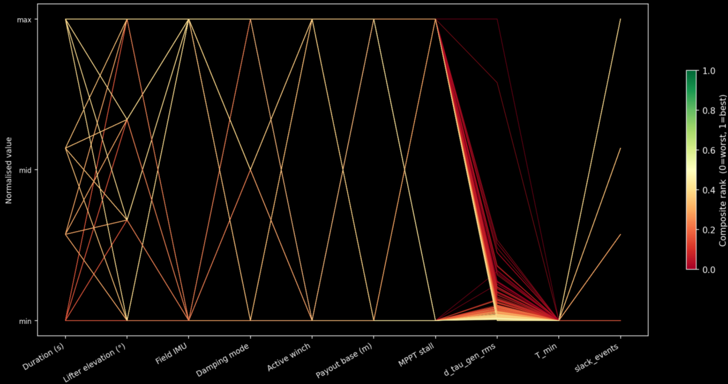
Parallel Coordinates — all 768 runs (each line = one run; colour = composite rank: green=best, red=worst)
