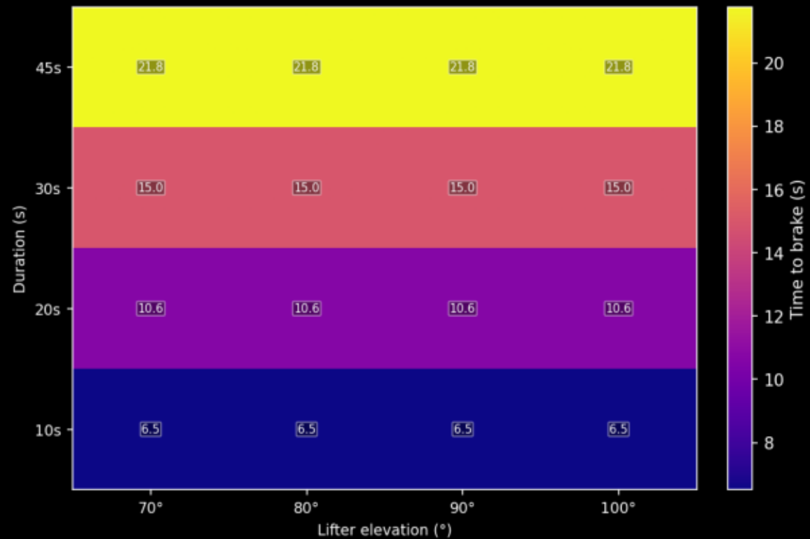
Mean time to brake (s) — duration × lifter elevation
