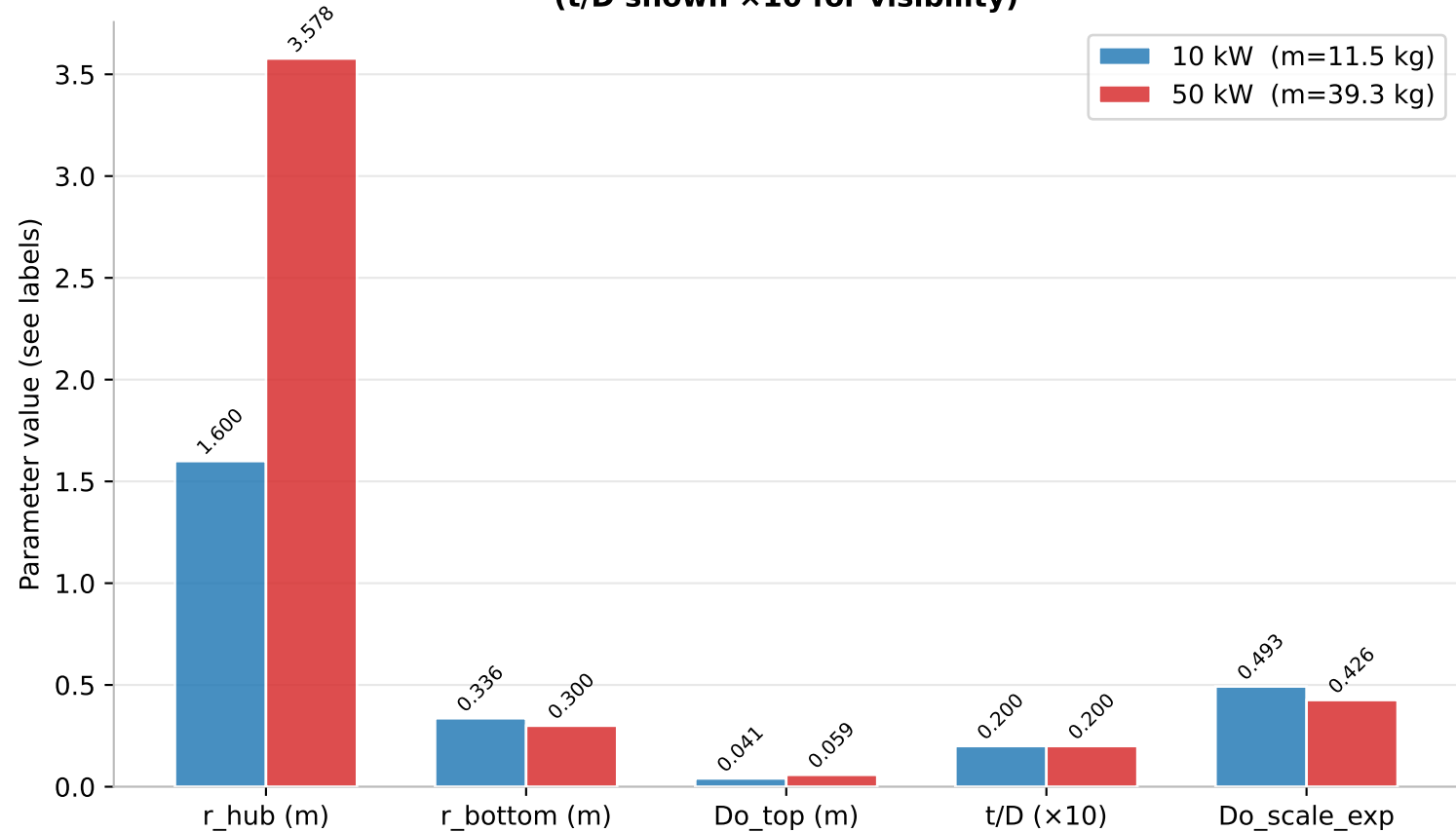
V5 Optimal Design Parameters — 10 kW vs 50 kW (t/D shown \times 10 for visibility)
