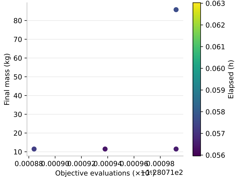
V5 10 kW Islands Final mass vs. evaluations
