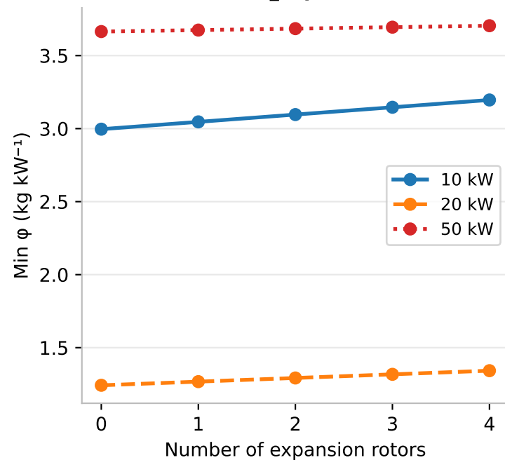
\phi monotonically increases with n_{\text{expansion}}
