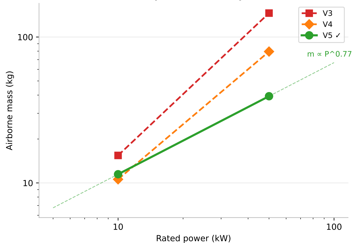
Mass vs Power Scaling (dotted = power-law extrapolation)
