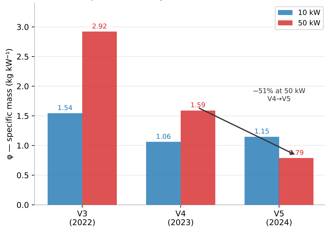
Specific Mass by Version & Power Class
