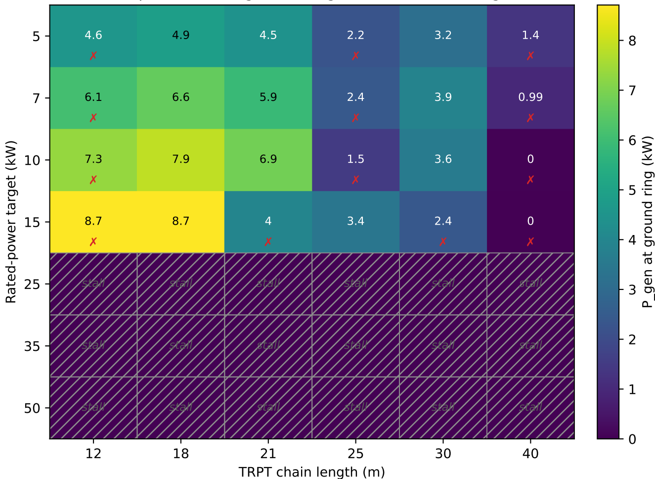
Delivered power at the ground ring — 42 baseline designs (v13)
