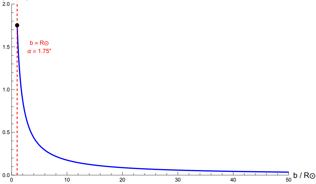
Deflection Angle vs. Impact Parameter (Solar Mass)
