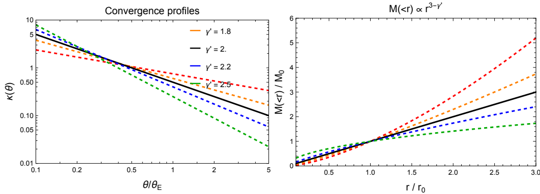
Figure 13.3: Power-law density profiles \rho \propto r^{-\gamma'} . Left: Convergence profiles for different slopes (the solid curve is the isothermal case \gamma' = 2 ). Right: Enclosed 3D mass M(\leq r) \propto r^{3-\gamma'} for the same slopes. Generated by galaxy_lensing.wl .
