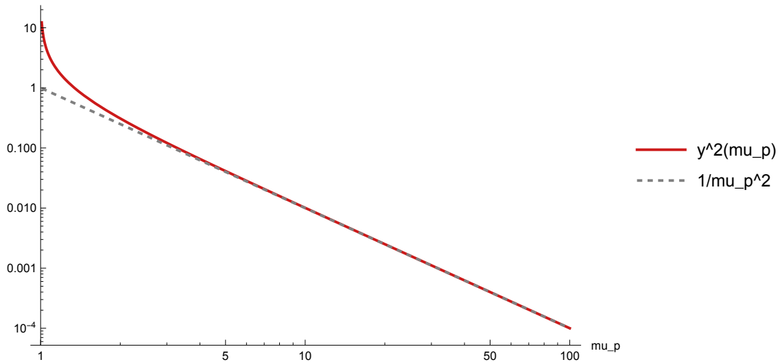
Point-mass magnification cross-section
