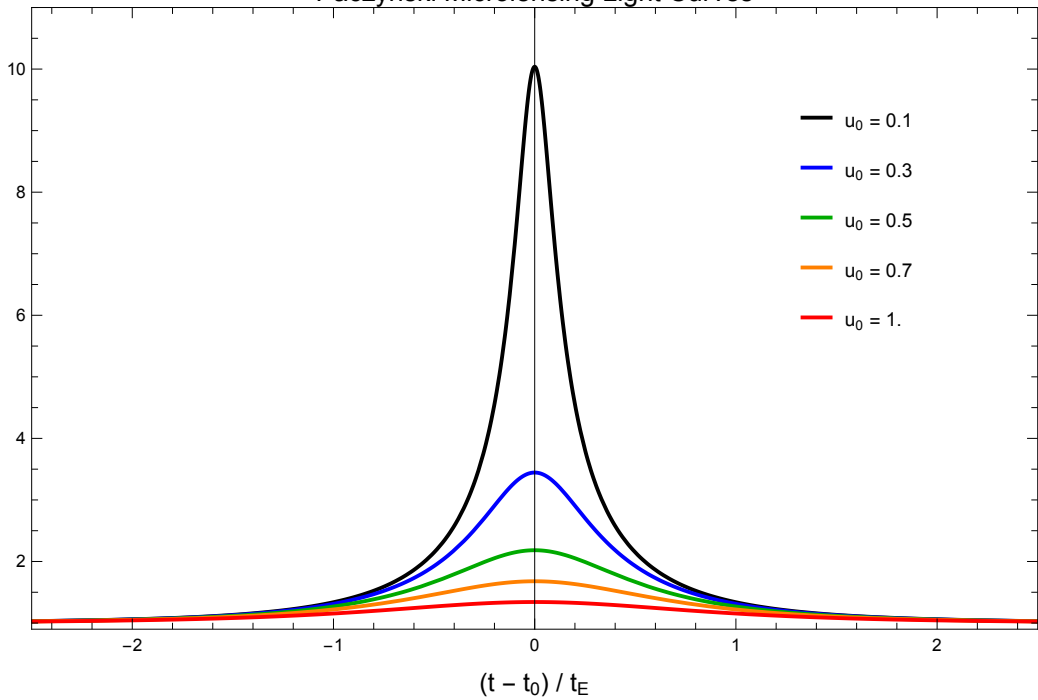
Paczynski Microlensing Light Curves
