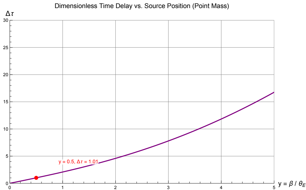
Figure 10.3: Dimensionless time delay \Delta\tau between the two images of a point mass lens as a function of the source position y = \beta/\theta_E . The time delay increases with the source offset. For y \rightarrow 0 (Einstein ring limit), \Delta\tau \rightarrow 0 because the two images become symmetric. Generated by time_delay_function.wl .
