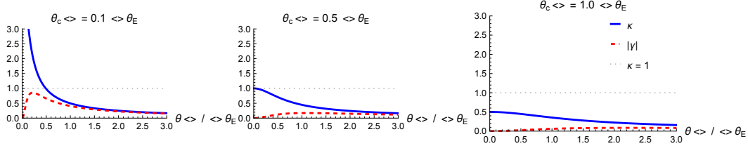
Figure 11.1: Effect of the core radius on NIS critical curves. Left: for \theta_c < \theta_E/2 , both tangential and radial critical curves exist, enabling three images. Center: at the critical value \theta_c = \theta_E/2 , the radial critical curve collapses to a point. Right: for \theta_c > \theta_E/2 , no critical curves exist and only one image forms. Generated by axisymmetric_models.wl .
