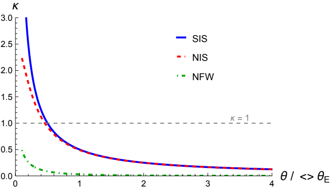
Convergence Profiles
