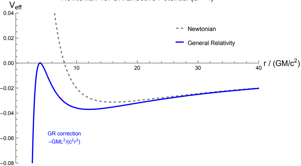
Newtonian vs. GR Effective Potential ( L = 4 )
