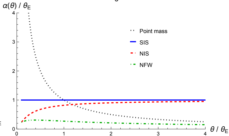
Deflection Angle Profiles
