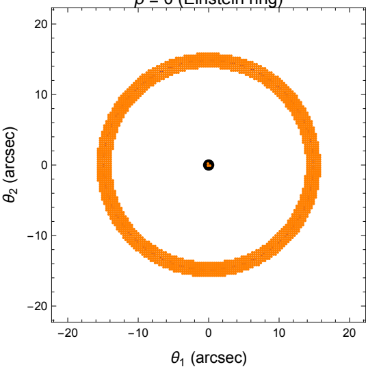
\beta = 0 (Einstein ring)
