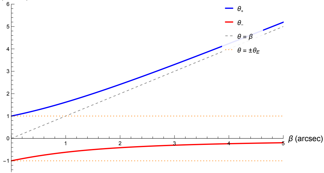
Image Positions (Exercise 4.5b)
