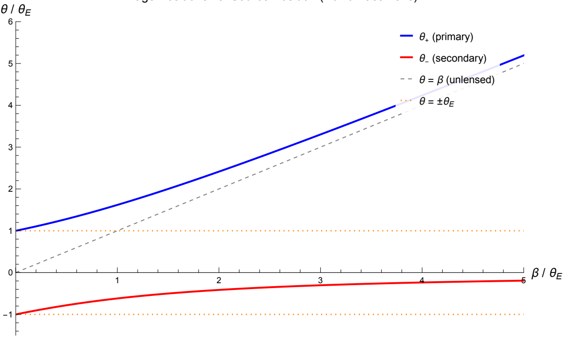
Image Positions vs. Source Position (Point Mass Lens)
