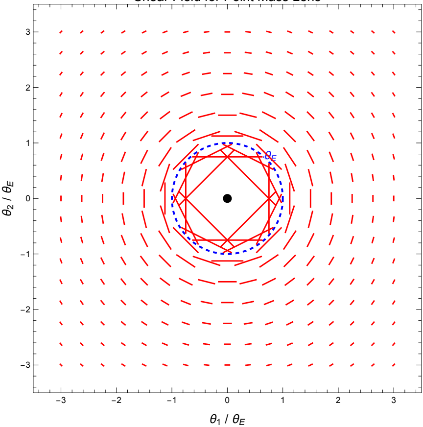
Shear Field for Point Mass Lens
