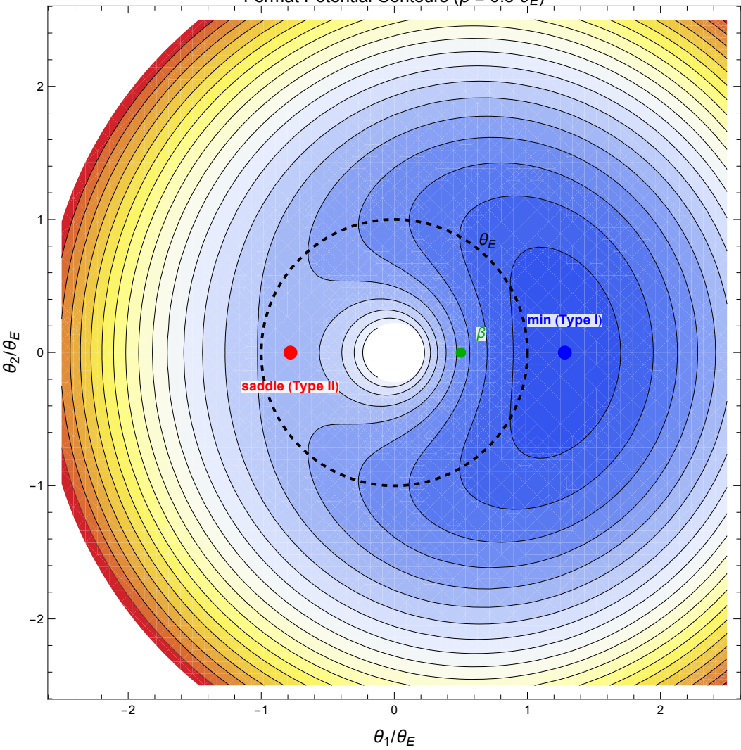
Fermat Potential Contours ( \beta = 0.5 \theta_E )
