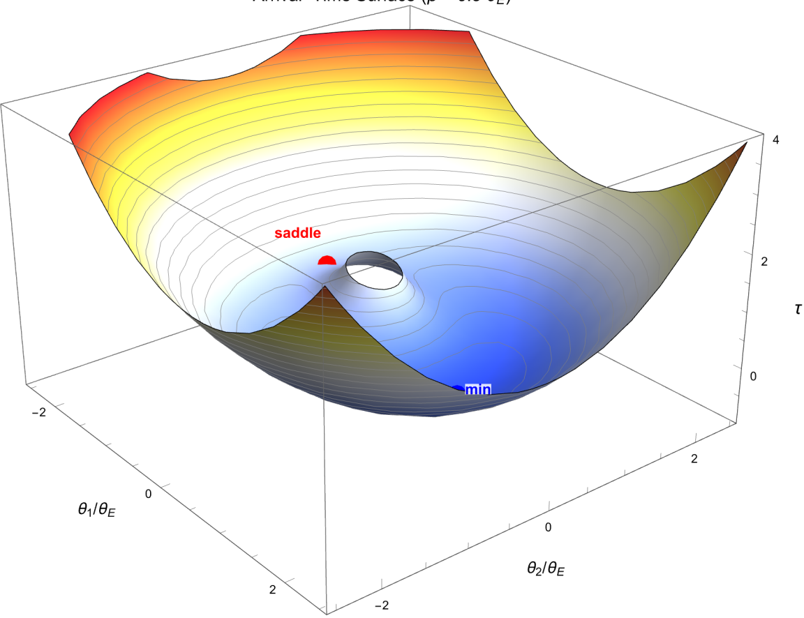
Arrival-Time Surface ( \beta = 0.5 \theta_E )
