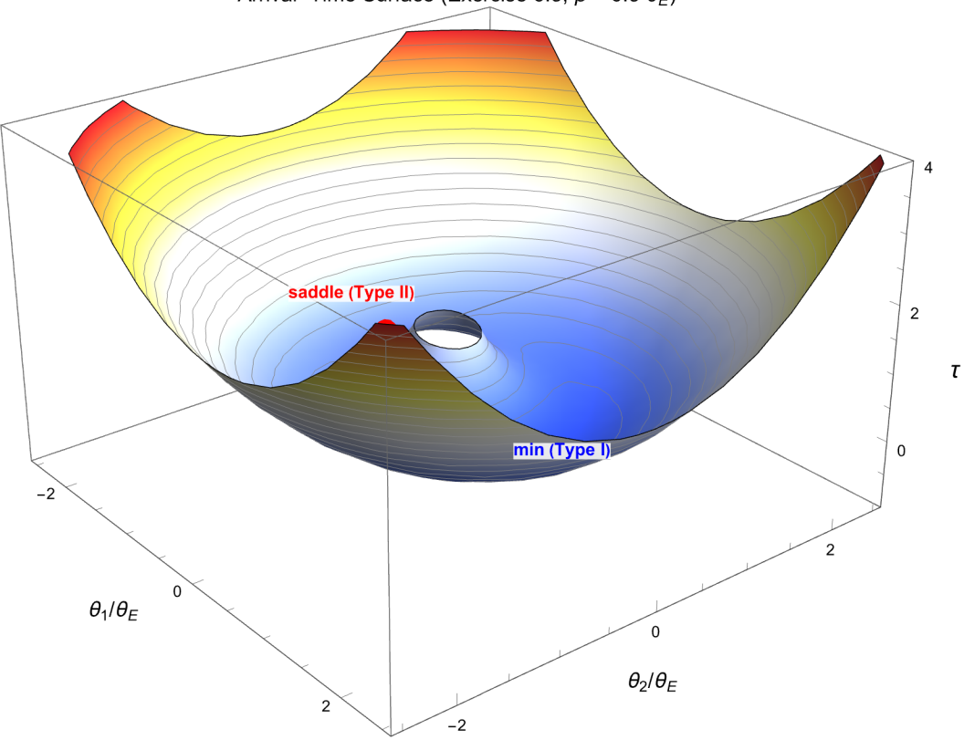
Arrival-Time Surface (Exercise 6.5, \beta = 0.3 \theta_E )
