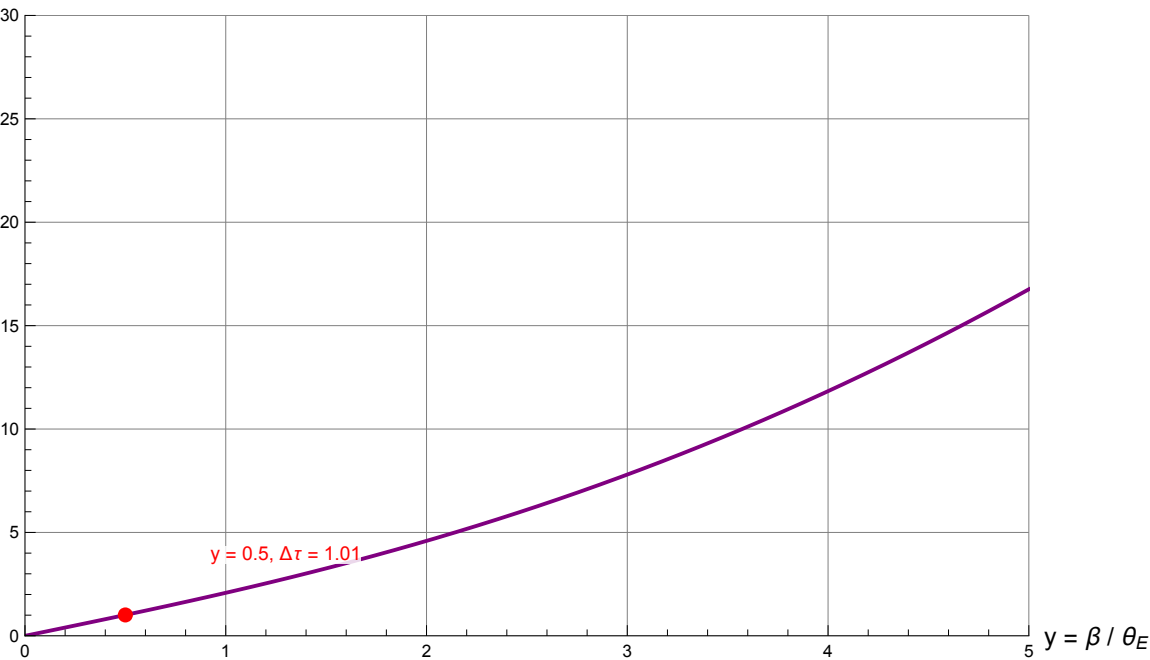
Dimensionless Time Delay vs. Source Position (Point Mass)
