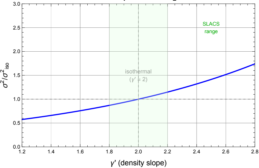
\sigma^2 vs \gamma' for fixed M_E
