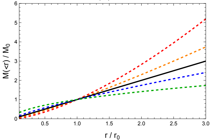
M(<r) \propto r^{3-\gamma'}
